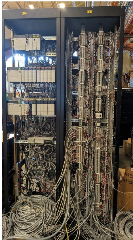
Fig.1 Rack B (left) and Rack A (right) rear views
